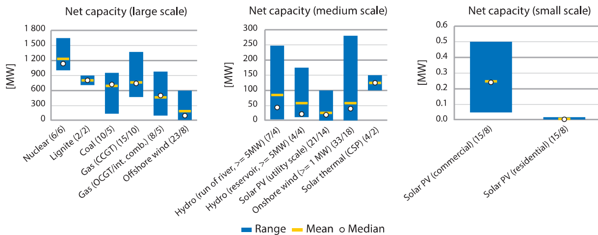
Figure 3.1: Range of capacity
