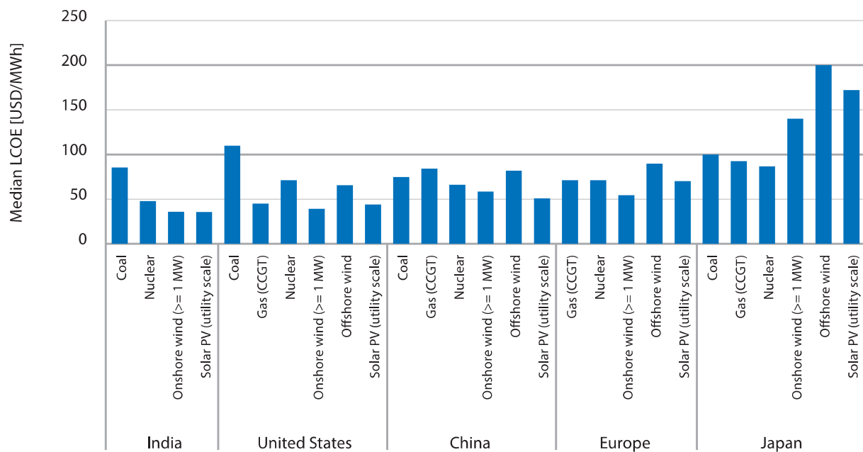
Figure 3.5: Median technology costs by region
