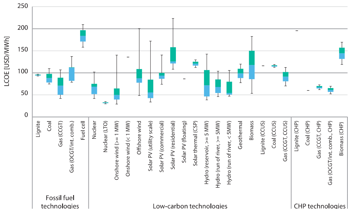
Figure 3.4: Overview of LCOE values
