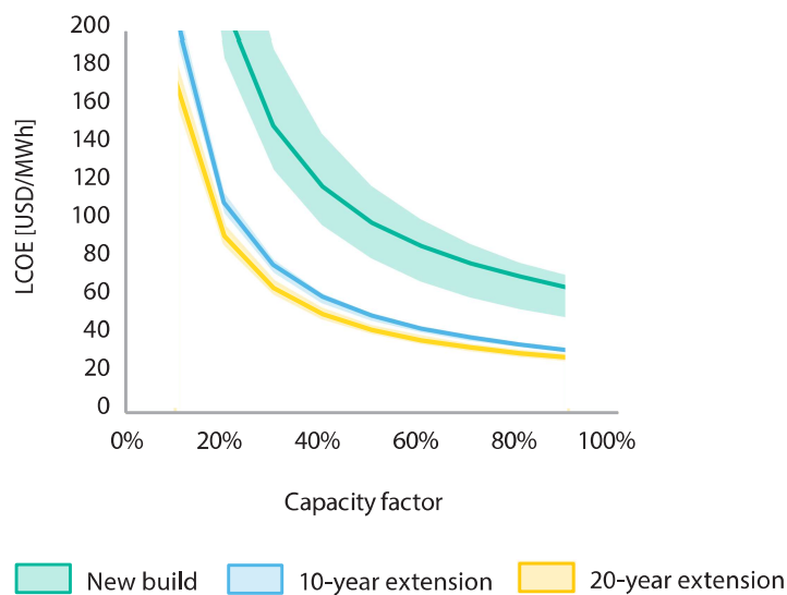
Figure ES3: Costs for nuclear new build and lifetime extension of existing plants
