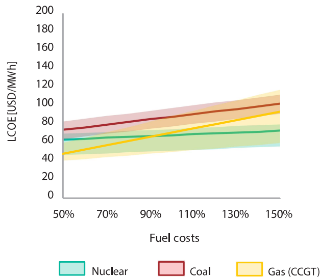
Figure 5.5: LCOE as a function of fuel cost
