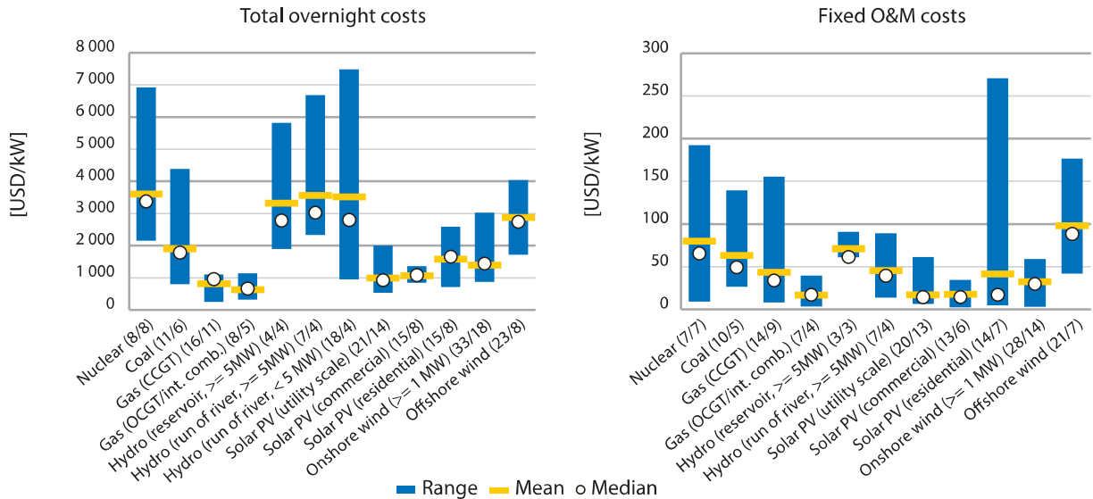
Figure 3.2: Range of overnight and fixed O&M costs
