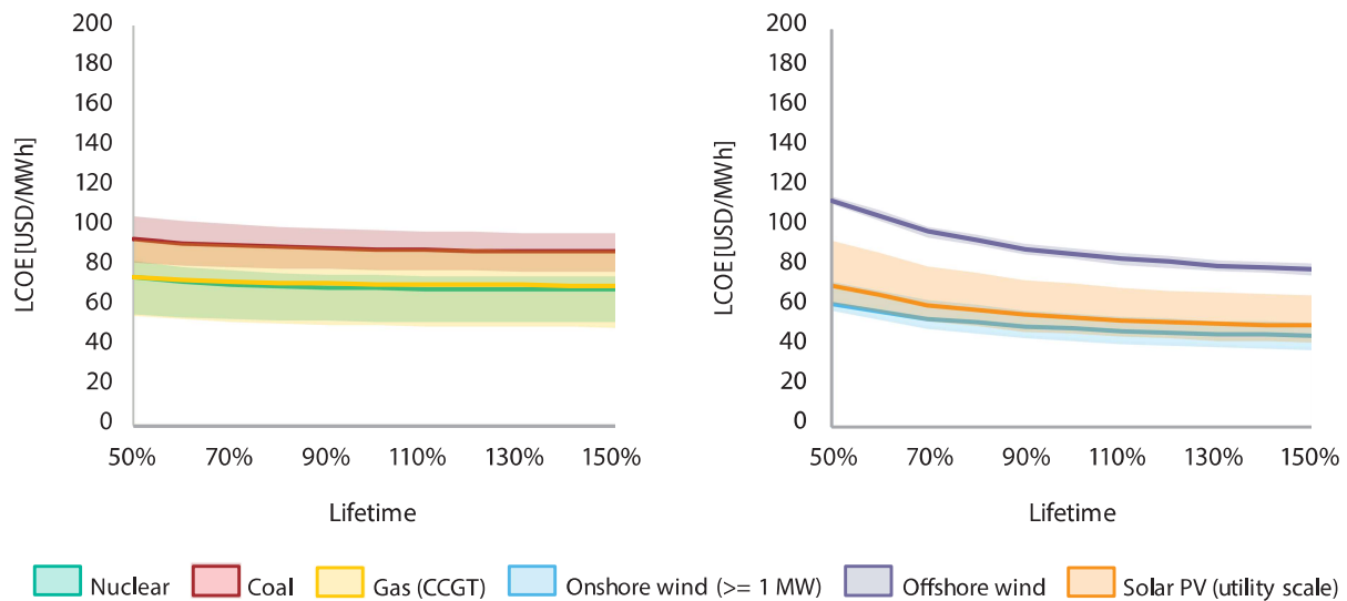
Figure 5.4: LCOE as a function of lifetime
