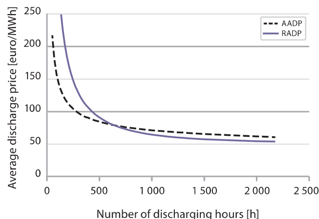
Figure 6.9: Comparison between the required and available average discharge price metrics, RADP and AADP, as a function of the number of discharge hours
