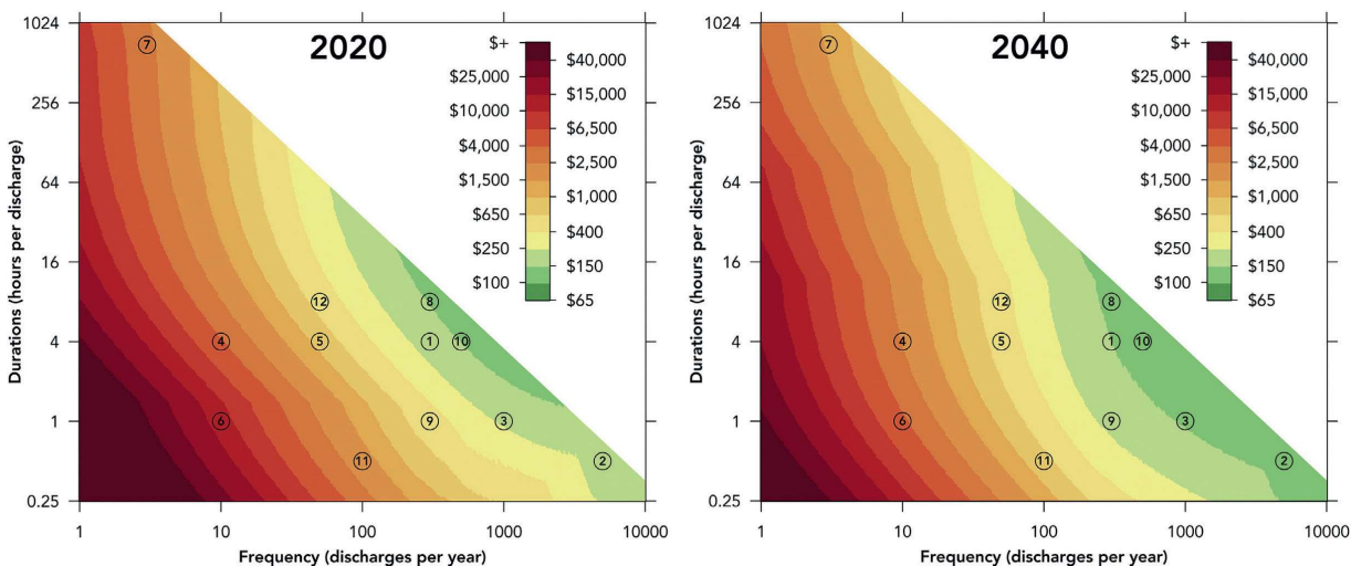
Figure 6.16: Projected levelised cost of the cheapest technologies displayed in a 2-D plot (number of annual cycles N_{cyc} , discharge duration \tau^d ) for the years 2020 and 2040
